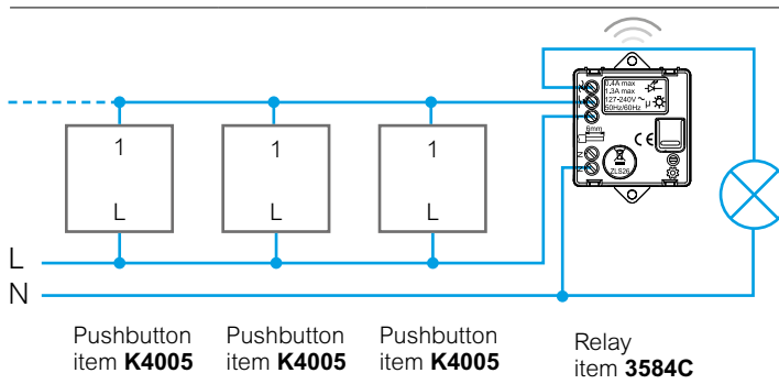
Three-point lighting control with pushbuttons and connected lighting micromodule, item 3584C, installed instead of a traditional relay
